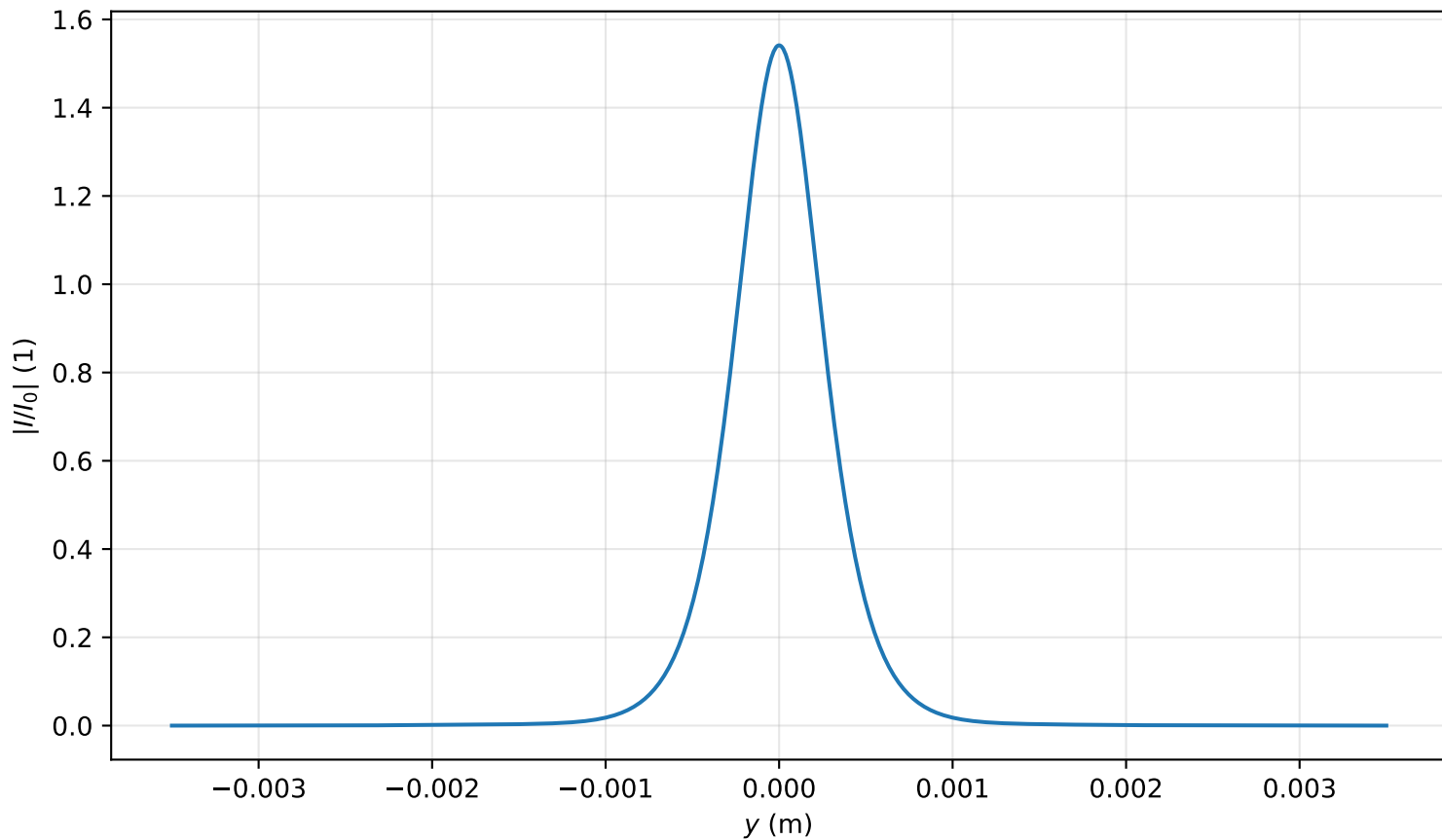
Intensity profile I(x=0, y, z=3.184)/I_0 , P_{in}=0.9P_{cr} , artificial time
